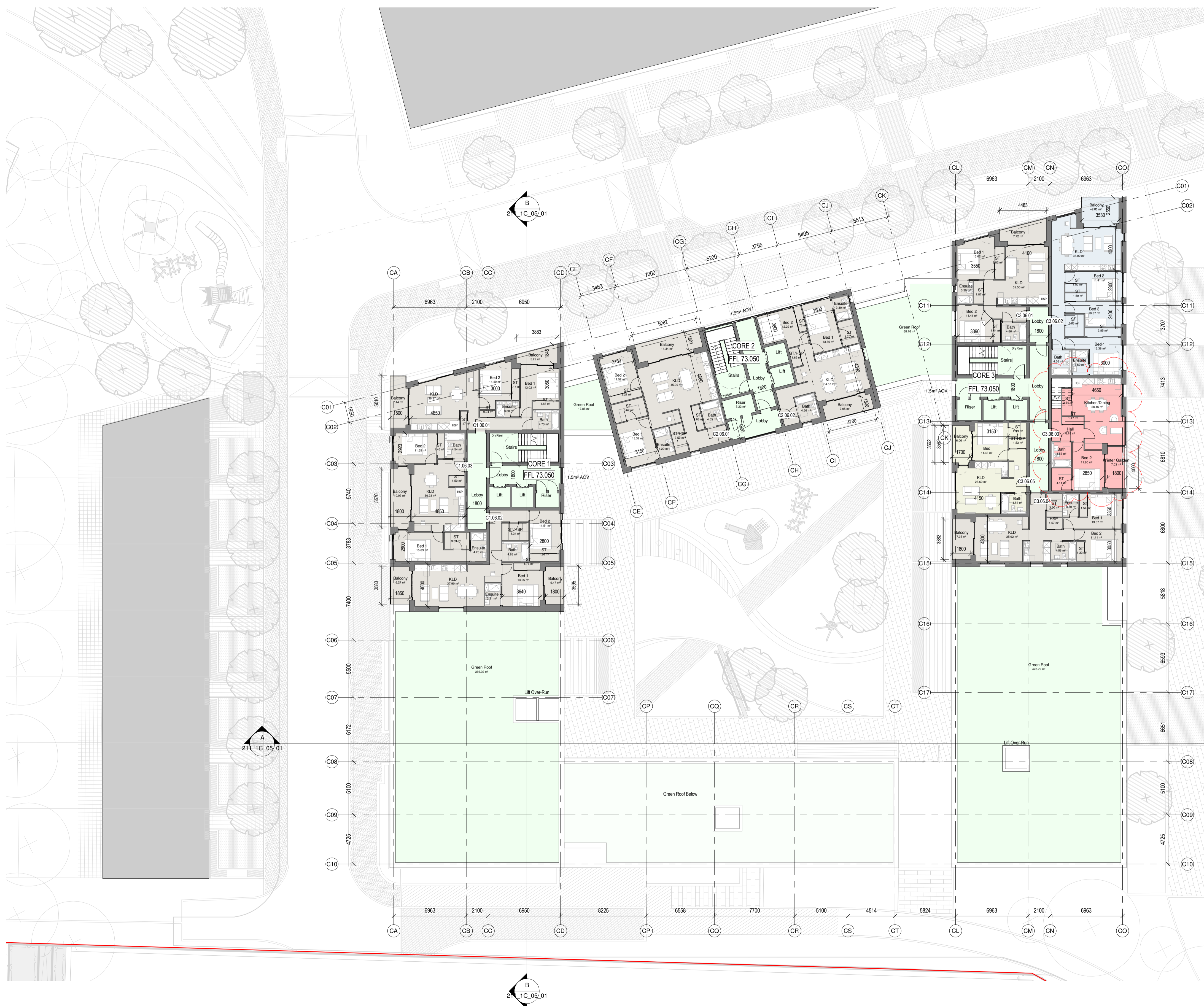
Block 1C_Sixth Floor Plan 1 : 200
