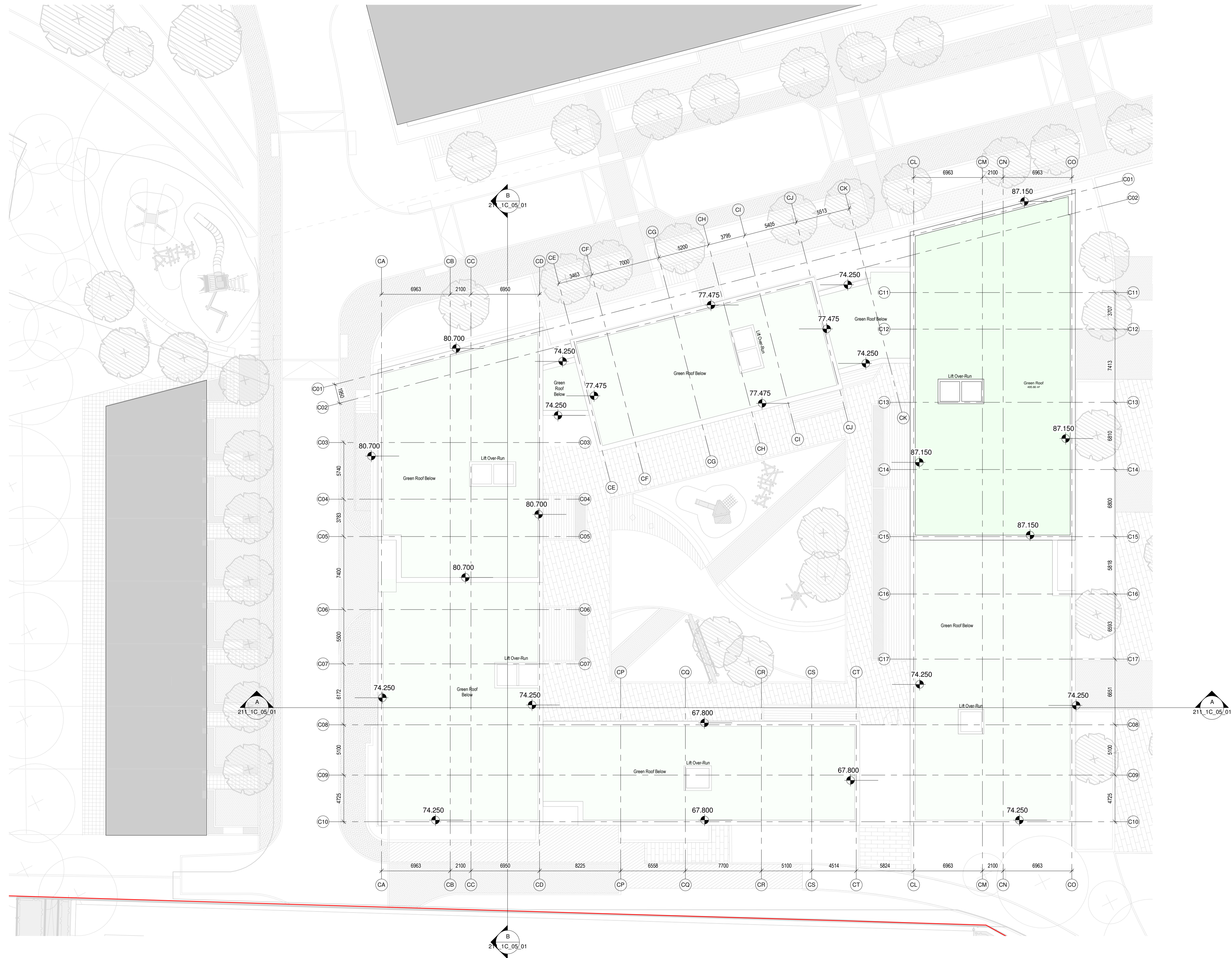
1 Block 1C_Roof Plan 1 : 200
