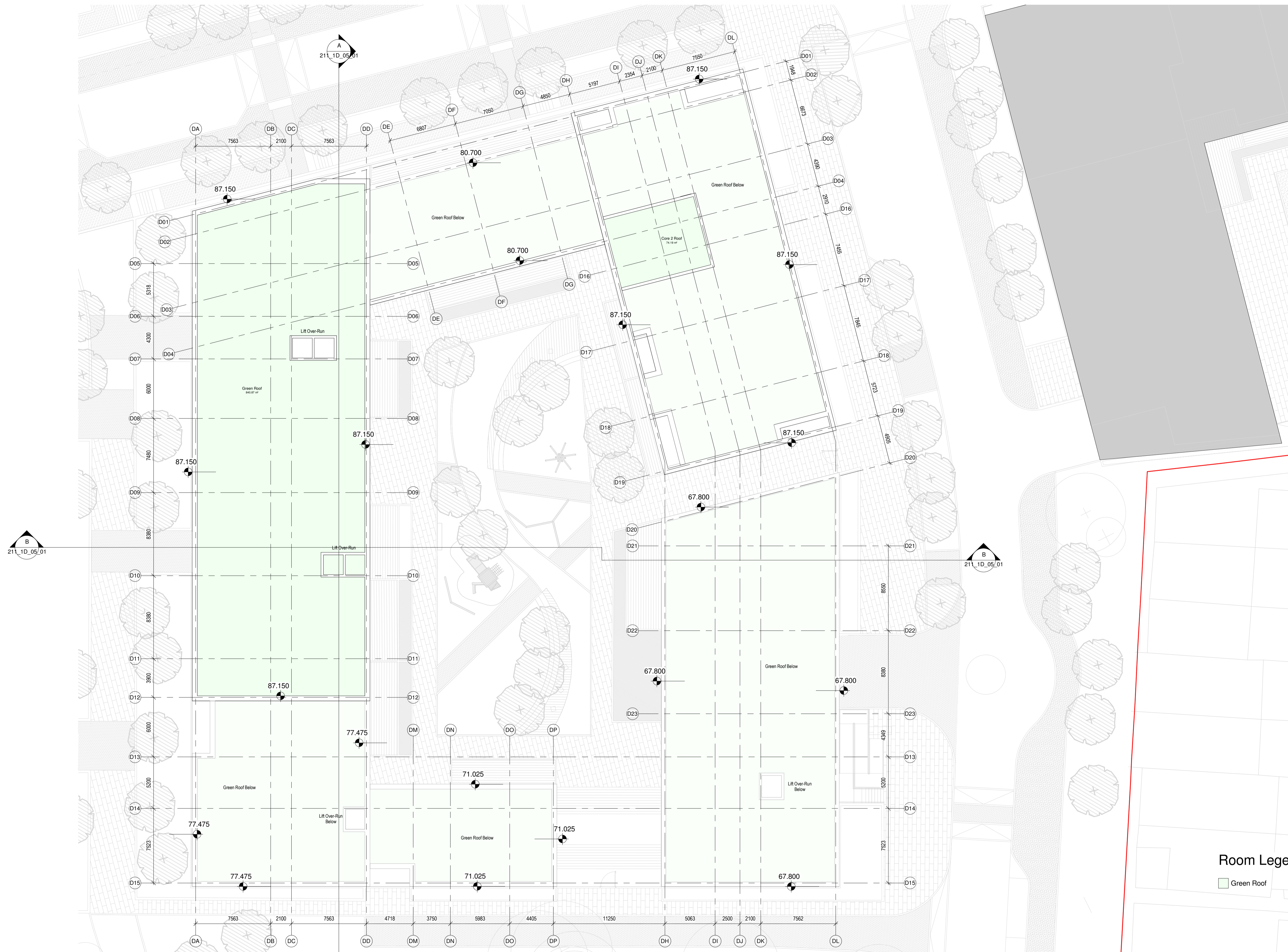
Block 1D_Roof Plan 1 : 200
