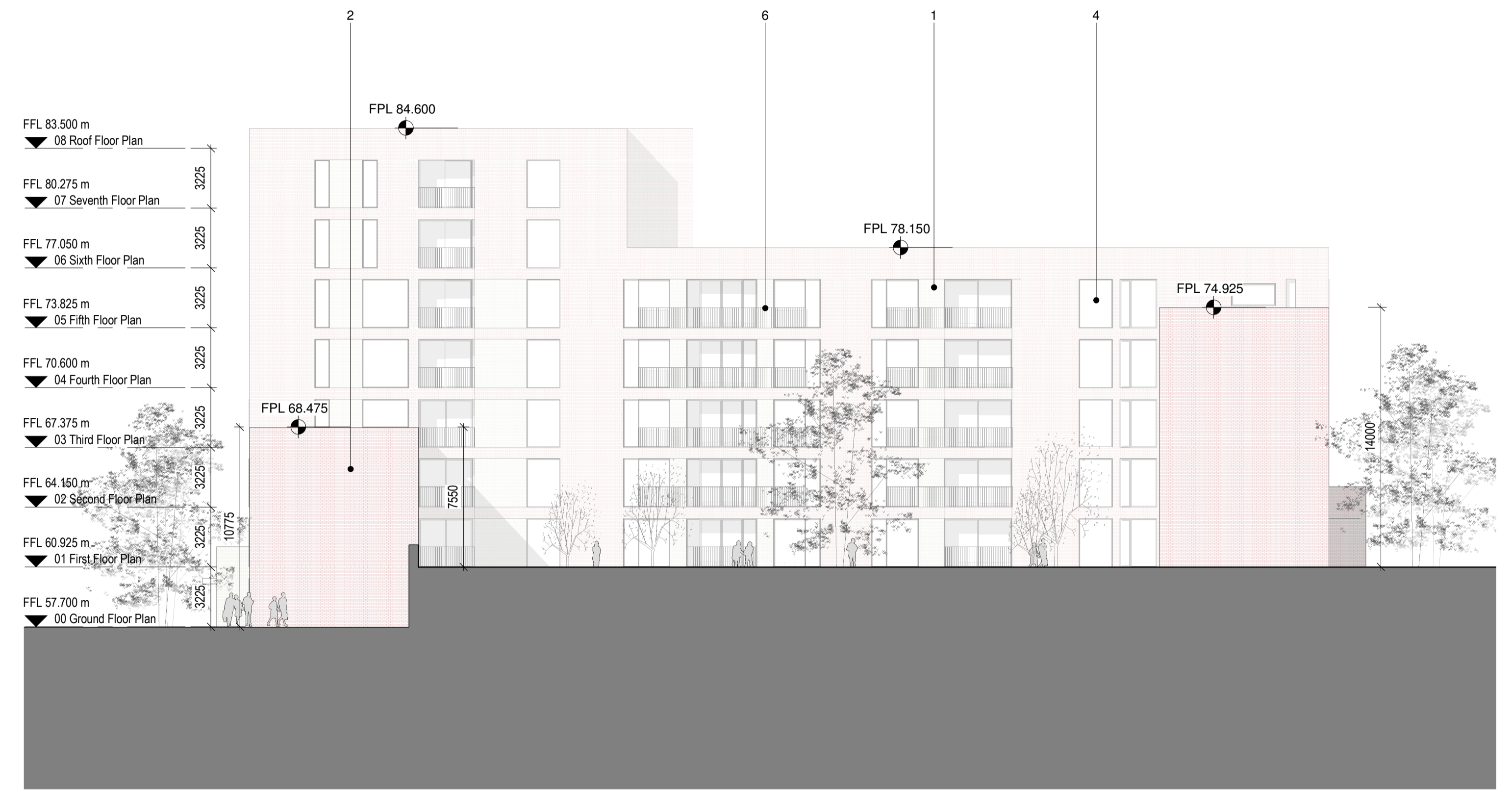
2 Block 1F_East Elevation 1 : 200
