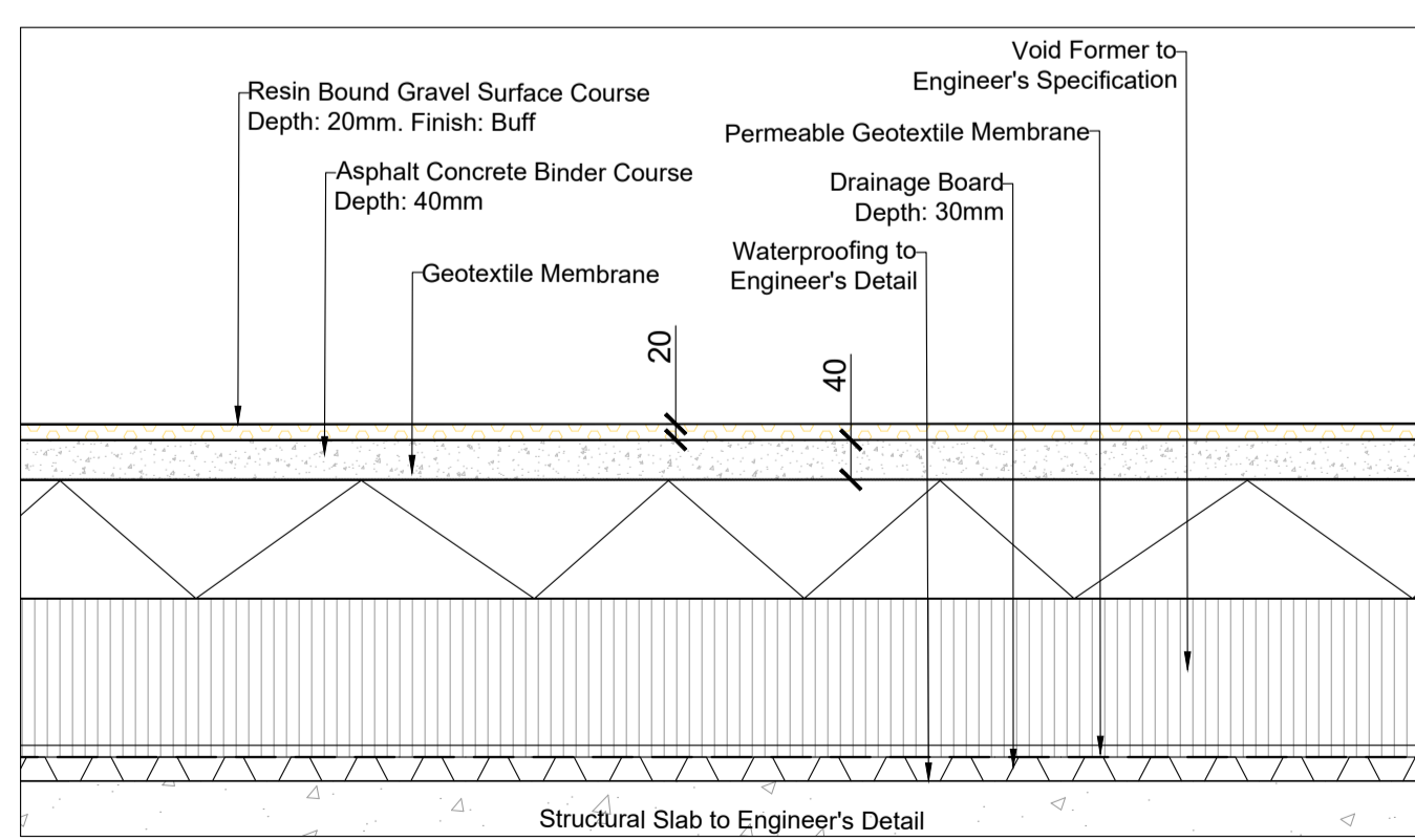
5 Resin Bound Gravel Surface - Over Structural Slab 1:10@A1
