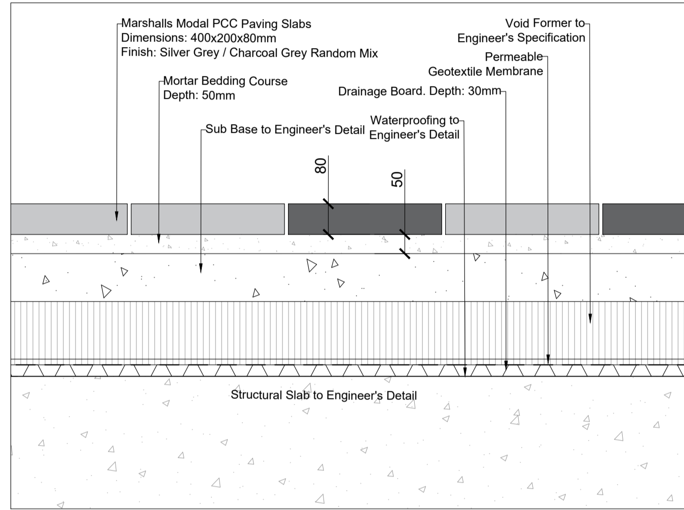
3 Paving Type 02 - Over Structural Slab 1:10@A1
