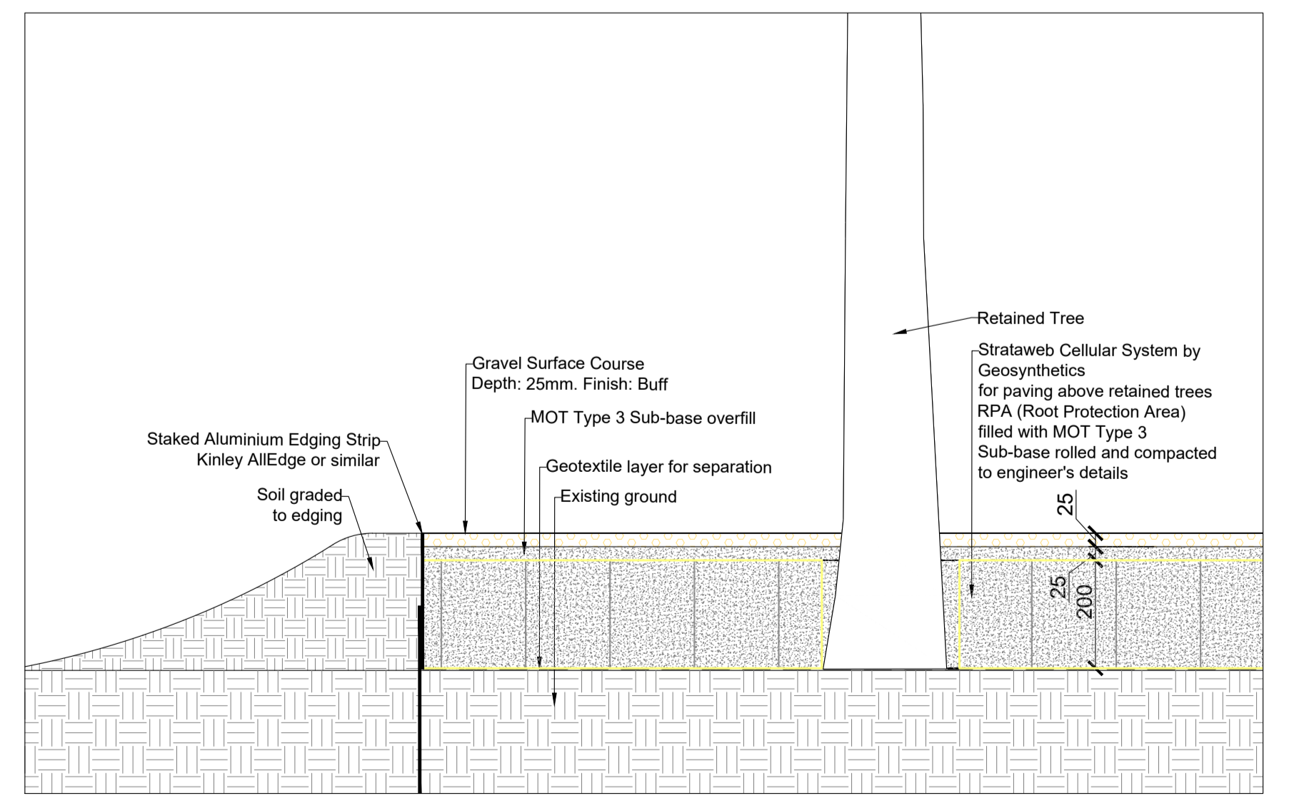
7 Gravel Surface - Over retained tree Root Protection Area 1:10@A1
