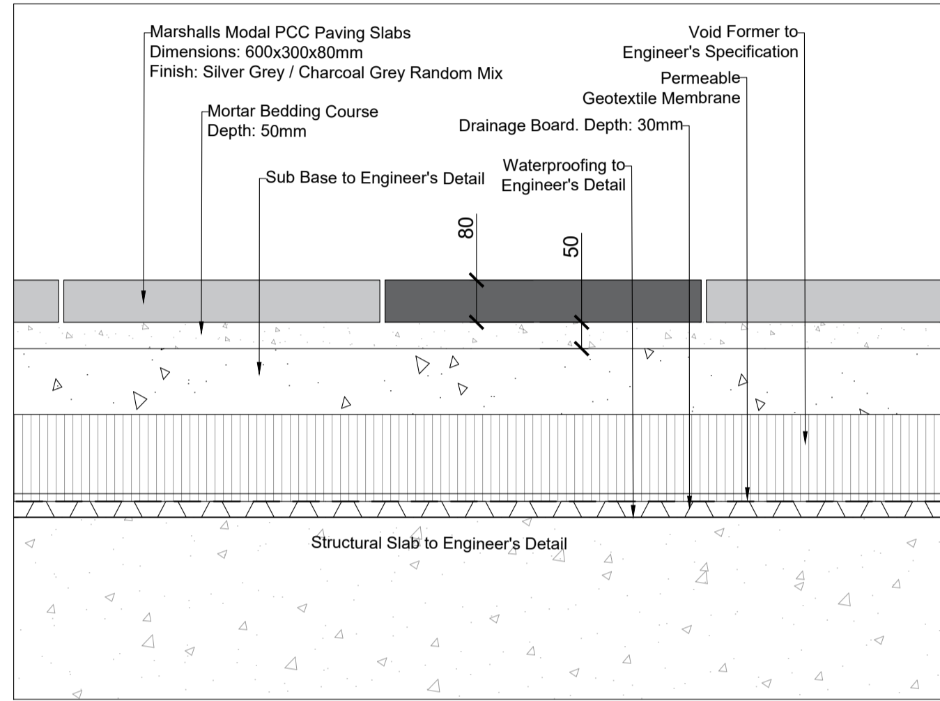
2 Paving Type 01 - Over Structural Slab 1:10@A1
