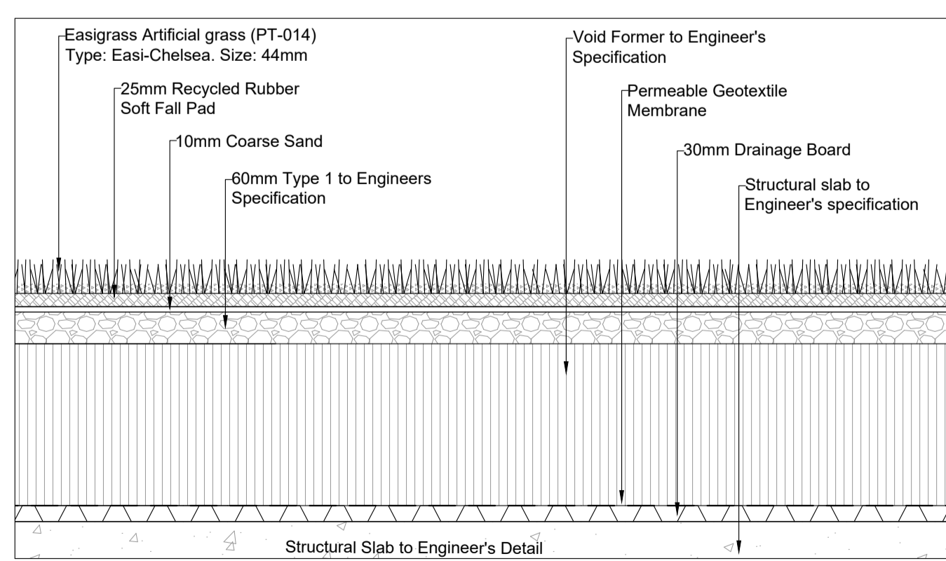
6 Artificial Grass Play Surfacing - Over Structural Slab in Courtyards 1:10@A1
