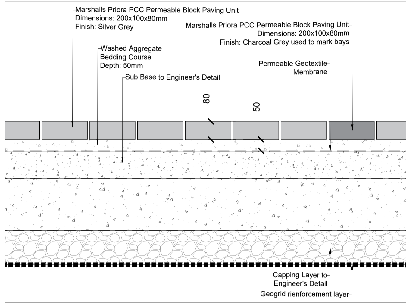
1 Paving Type 05 1:10@A1
