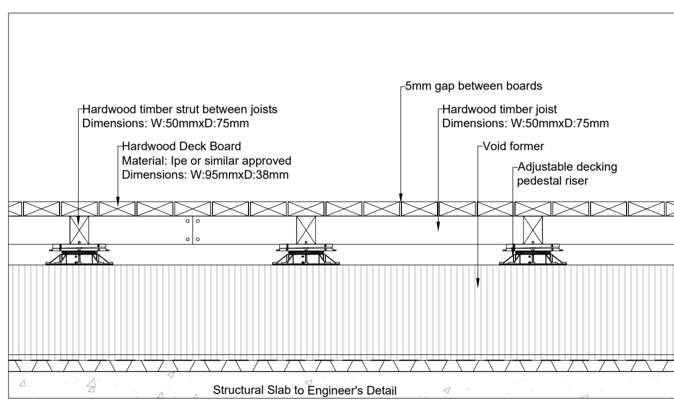
4 Hardwood Timber Decking - Over Structural Slab 1:10@A1
